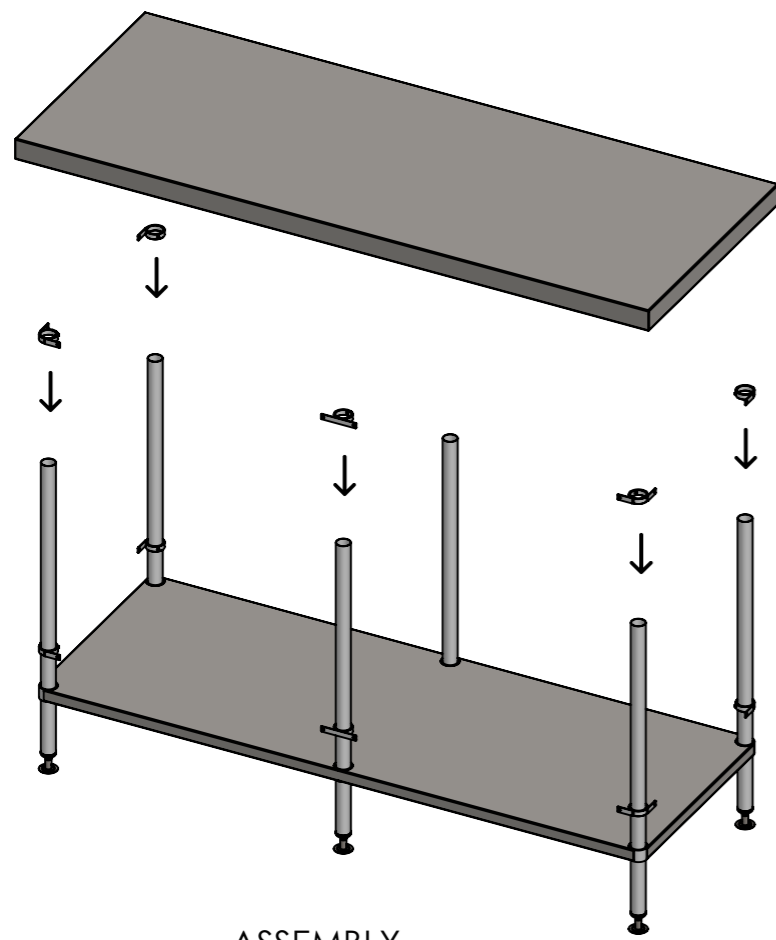
ASSEMBLY
